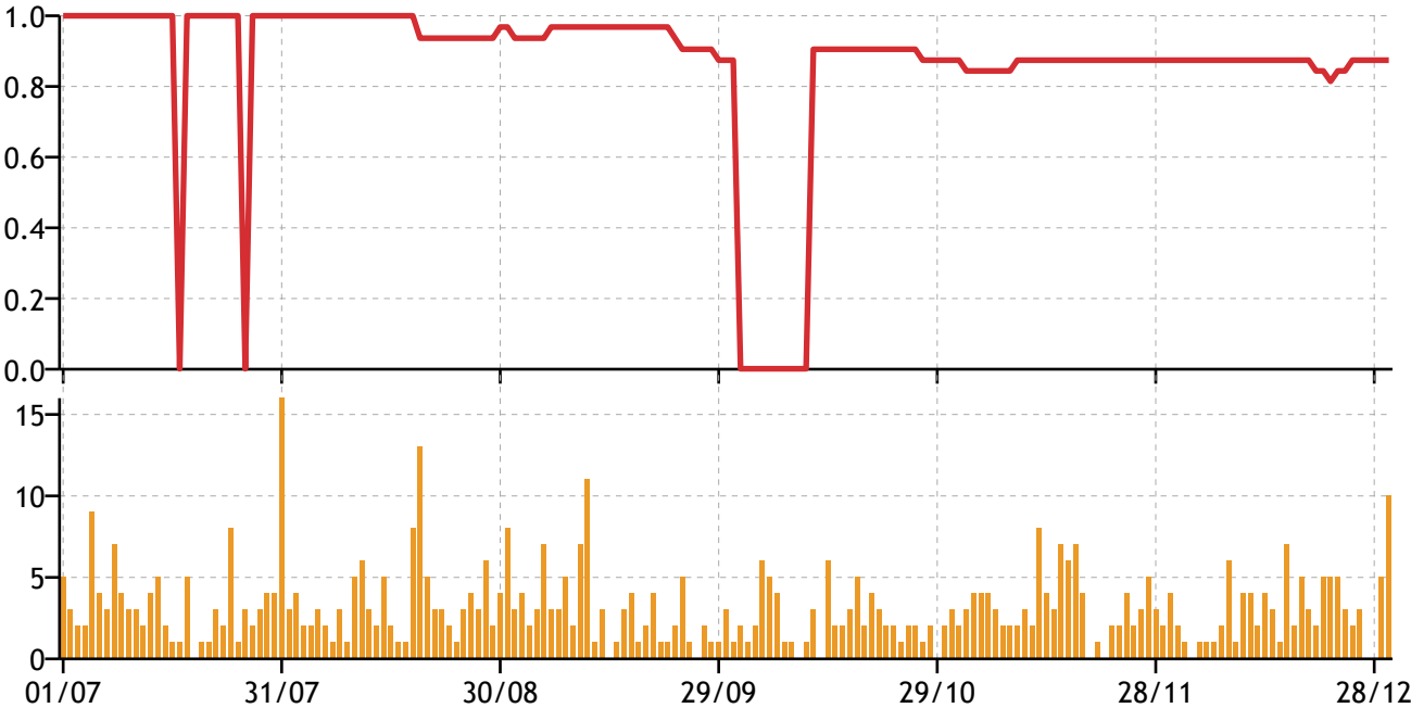
Figure 10: Muse Chart Popularity vs Twitter Coverage
