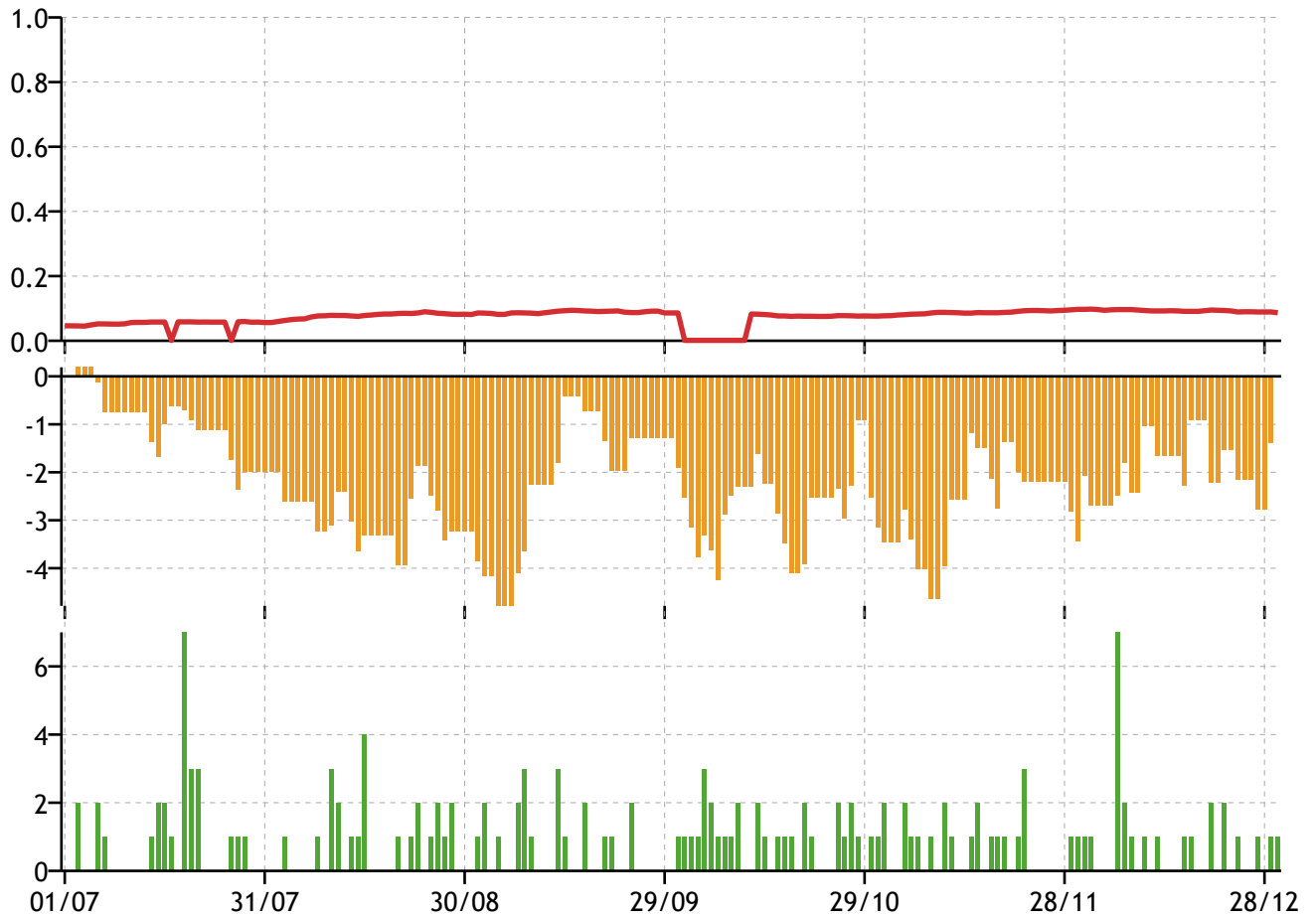
Figure 13: McFly Chart Popularity vs News Sentiment + Volume
