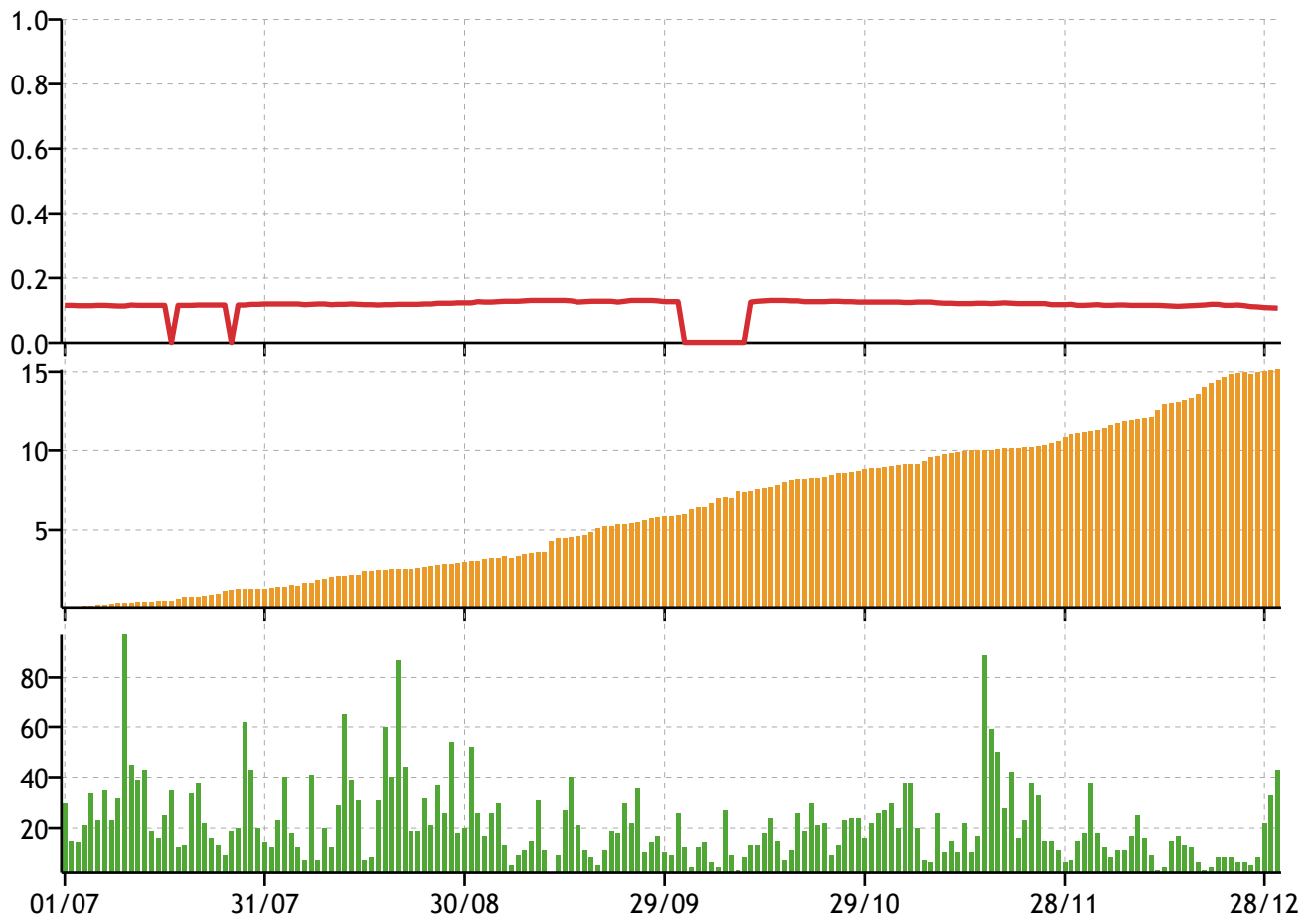
Figure 20: Jay-Z Chart Popularity vs News Sentiment + Volume
