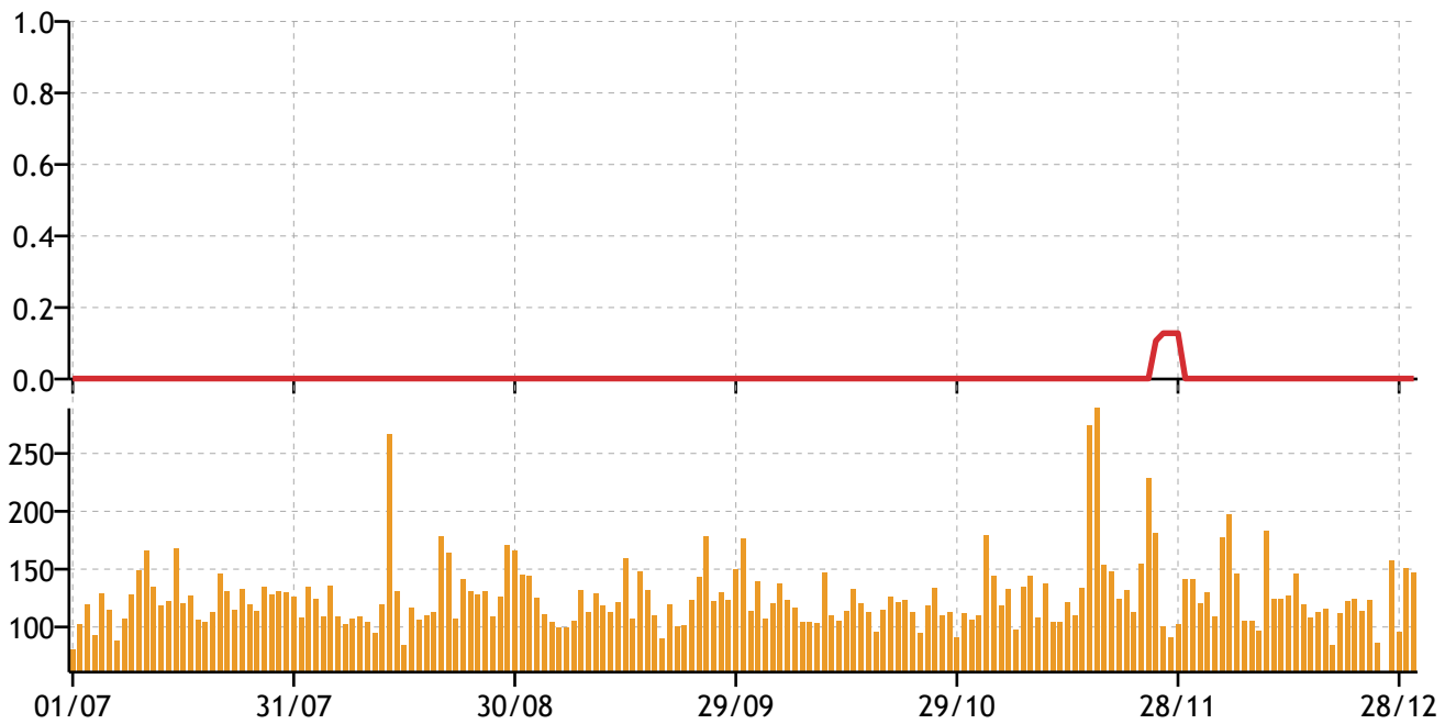
Figure 14: Jay-Z Chart Popularity vs Twitter Coverage
