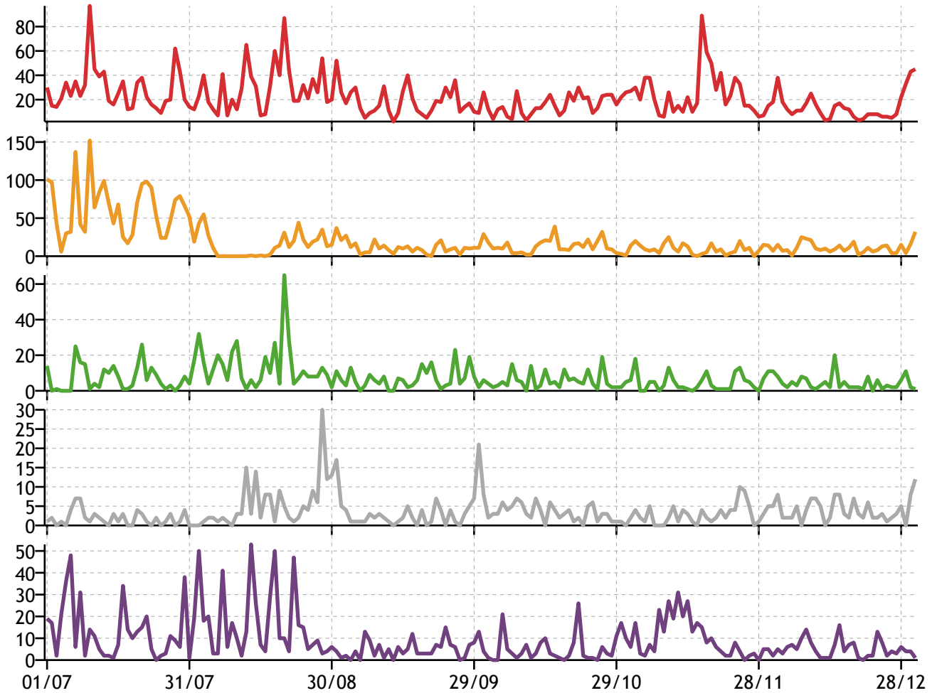
Figure 19: Comparisons for Jay-Z
