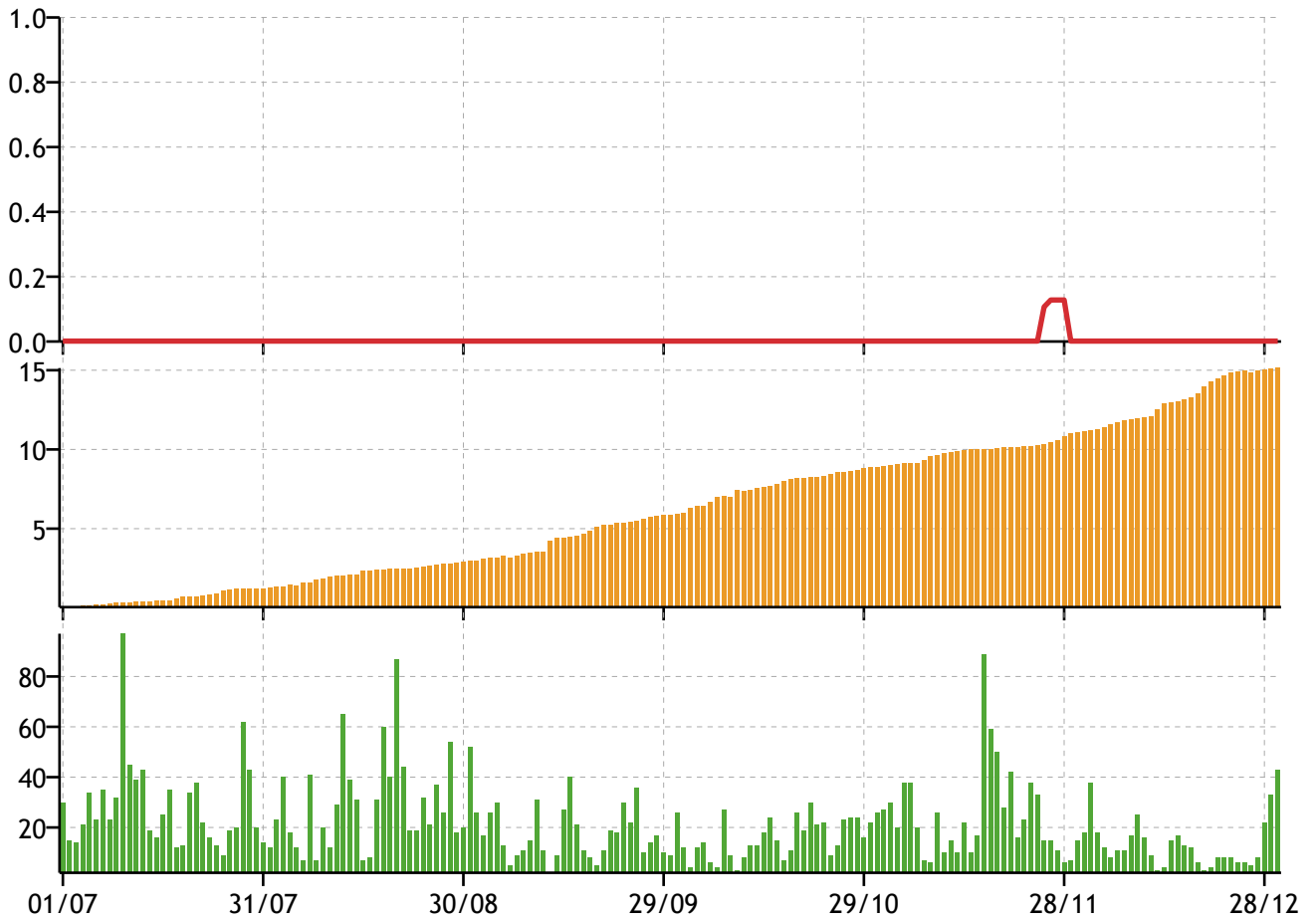
Figure 21: Jay-Z Chart Popularity vs News Sentiment + Volume
