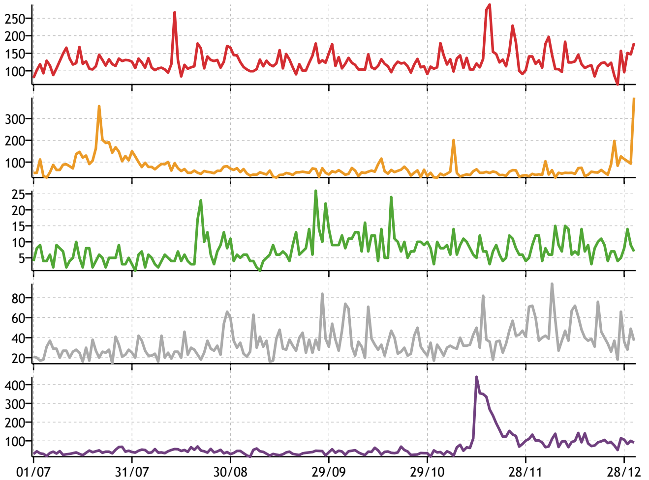
Figure 12: Comparisons for Jay-Z
