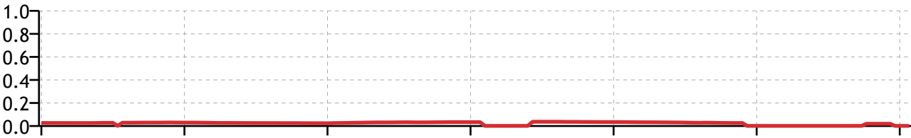
Figure 9: Chart ranking for Jay-Z
