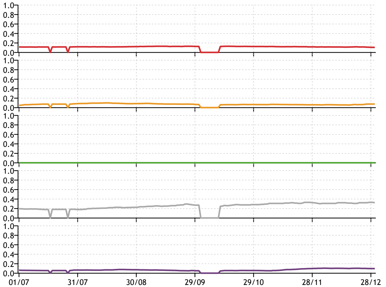
Figure 3: Comparisons for Jay-Z
