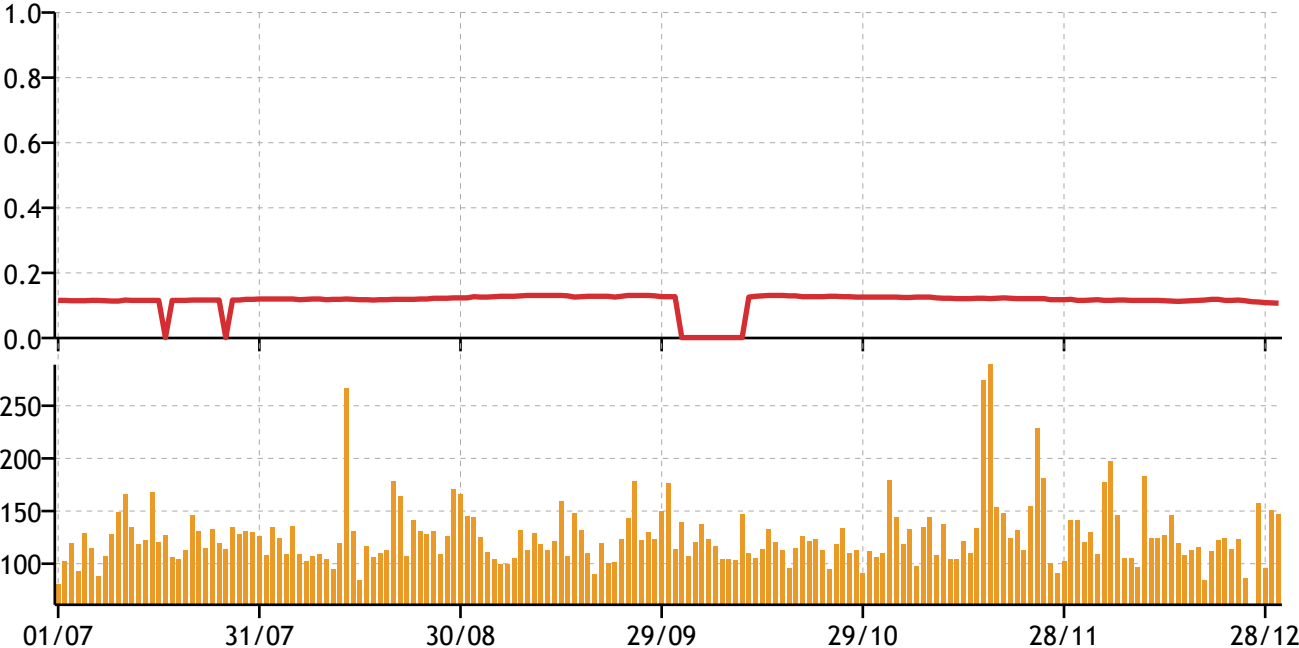
Figure 13: Jay-Z Chart Popularity vs Twitter Coverage
