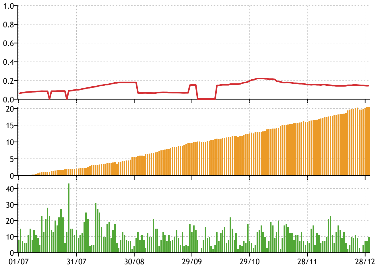
Figure 16: Flo Rida Chart Popularity vs News Sentiment + Volume
