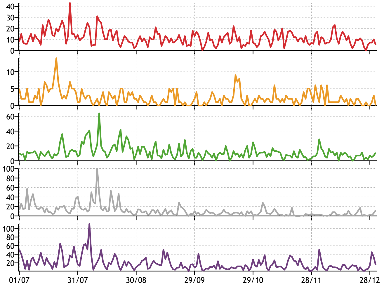
Figure 15: Comparisons for Flo Rida
