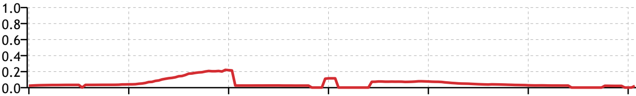
Figure 6: Chart ranking for Flo Rida
