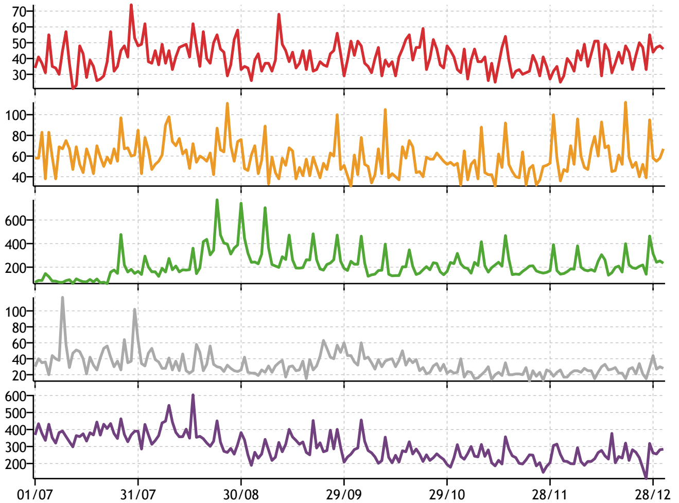
Figure 9: Comparisons for Flo Rida
