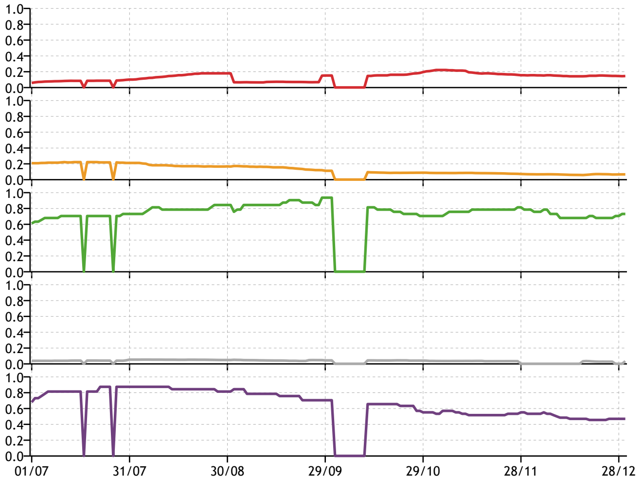
Figure 3: Comparisons for Flo Rida
