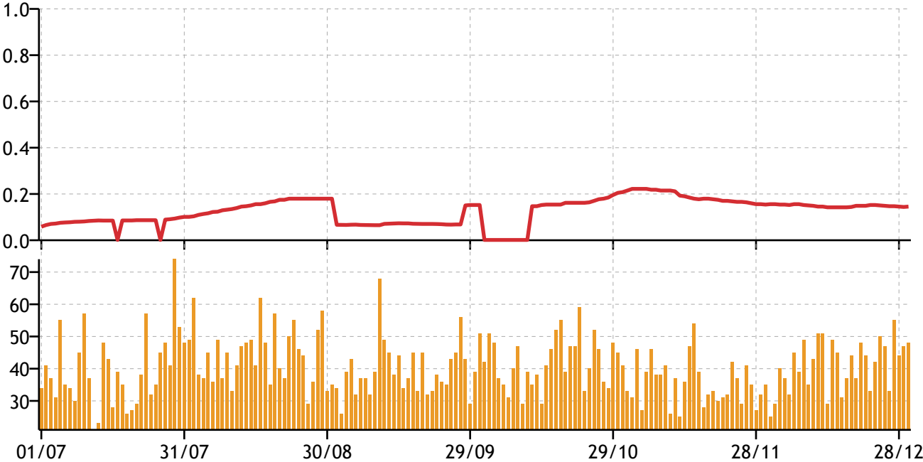
Figure 10: Flo Rida Chart Popularity vs Twitter Coverage
