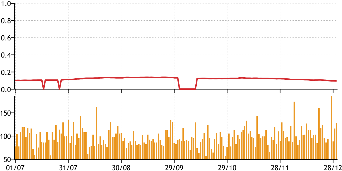
Figure 10: Depeche Mode Chart Popularity vs Twitter Coverage
