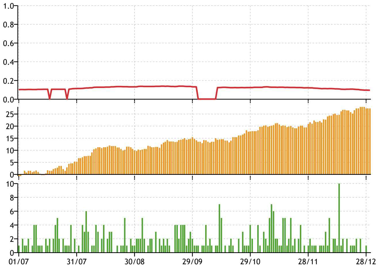
Figure 16: Depeche Mode Chart Popularity vs News Sentiment + Volume
