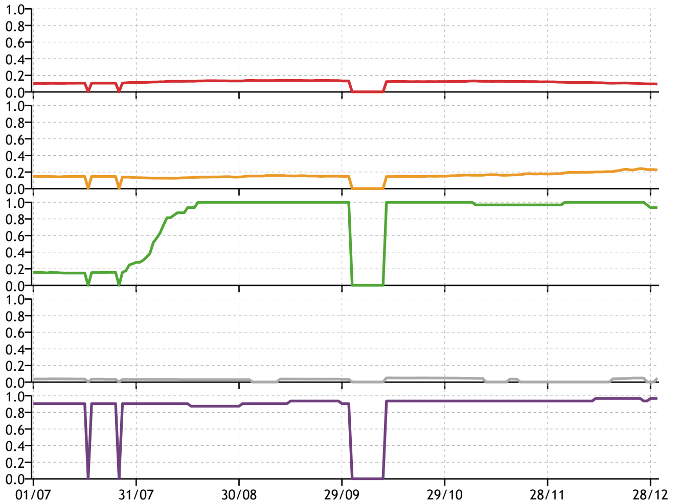
Figure 3: Comparisons for Depeche Mode
