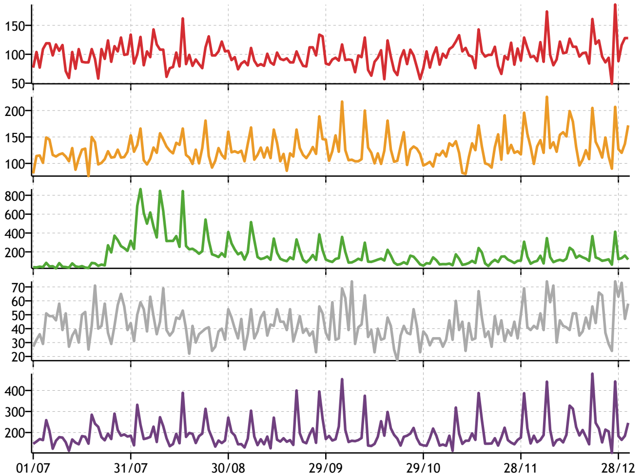
Figure 9: Comparisons for Depeche Mode
