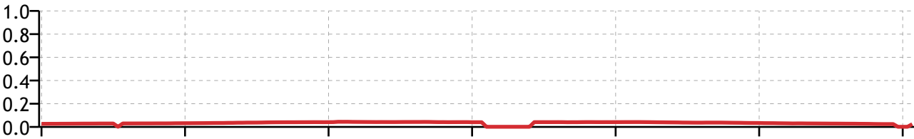
Figure 6: Chart ranking for Depeche Mode
